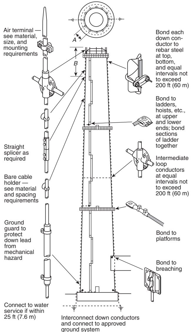
FIGURE 6.1 Heavy-Duty Stack.
