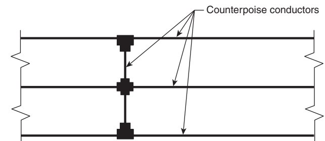
FIGURE 11.4.3.3 Multiple Counterpoise Conductor Installation Interconnection — Plan View.
