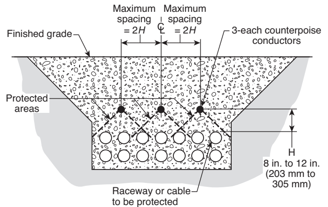
FIGURE 11.4.3.2 Multiple Airfield Lighting Raceways or Cables in a Common Formation.
